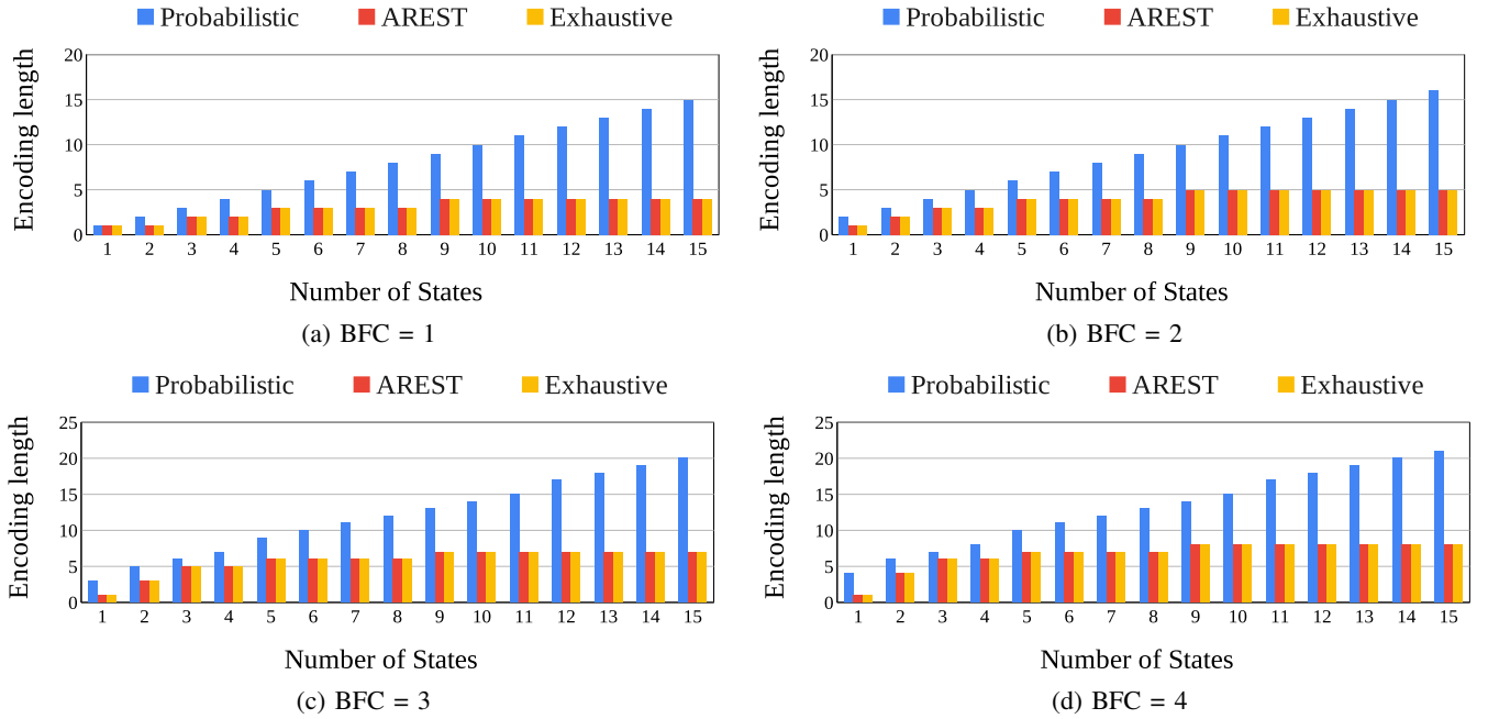
Figure 7: Generated encoding length comparison of proposed work AREST with Exhaustive [22] and Probabilistic [21] techniques for four different BFC values
