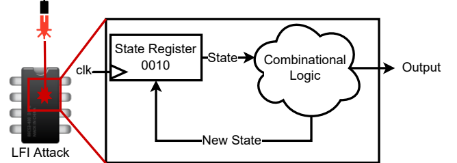
Figure 1: FSM hardware implementation with a state register and associated combinational logic.
