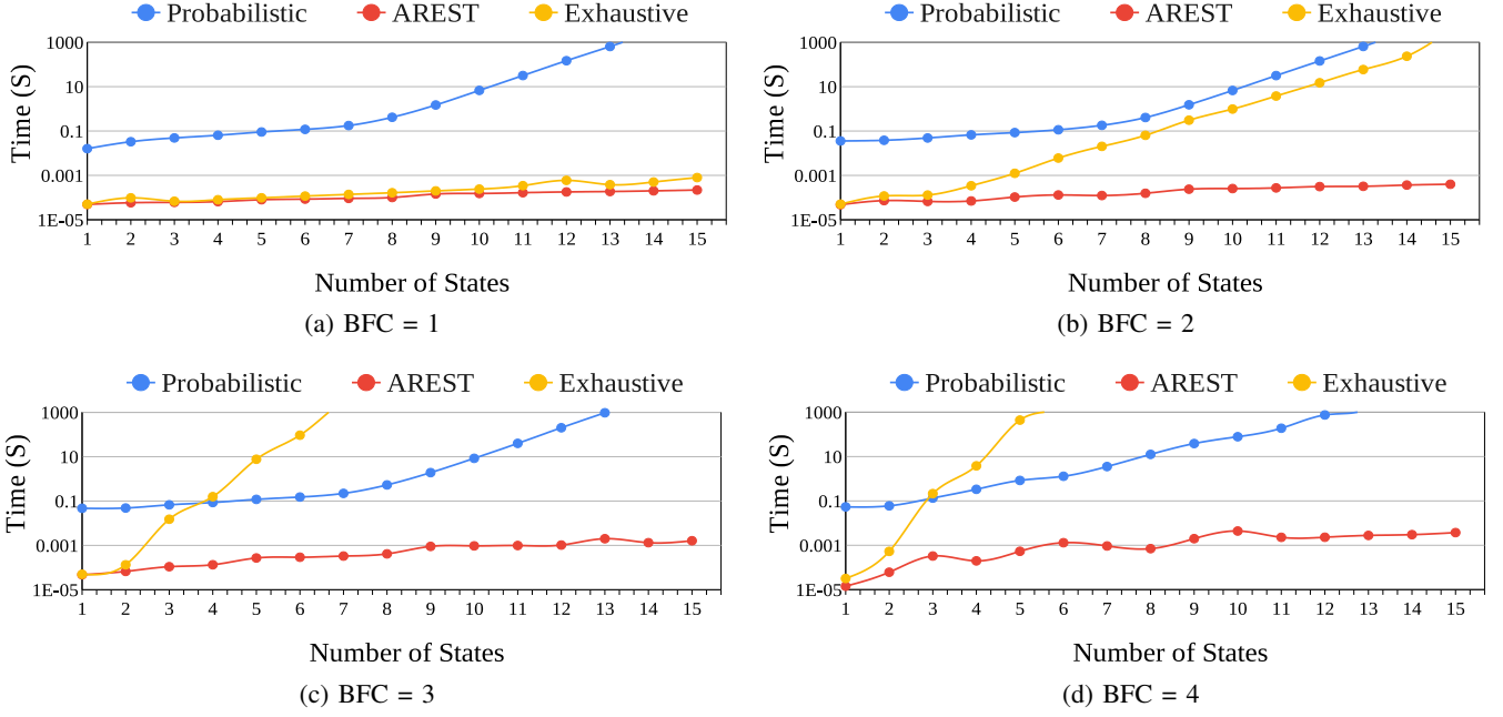
Figure 6: Runtime comparison of AREST with Exhaustive [22] and Probabilistic [21] techniques for four different BFC values
