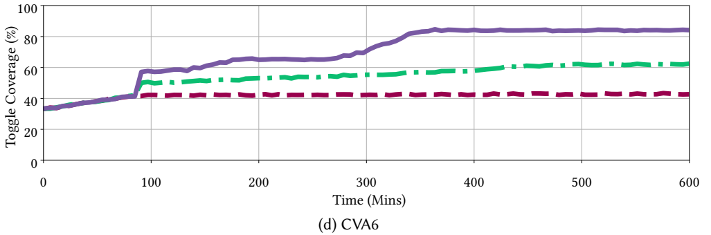
Fig. 11. Toggle coverage results of FuSS compared with traditional fuzzing and fuzzing with property checking.
