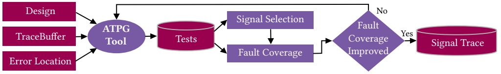
Fig. 20. Observability-aware test generation for detecting electrical errors [7]
