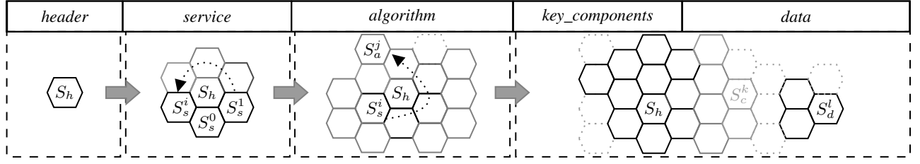
Fig. 9: Illustration of the growth of state space based on a request packet from the host system to RoT via shared memory. Each parameter in the packet contributes to the increase in the state space. Note that this is an example of a single request. In reality, the RoT firmware kernel runs several threads serving multiple host requests at a time, which can lead to state explosion.
