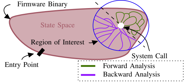
(b) Proposed system call directed symbolic execution creates intermediate entry points for each system call to mitigate state explosion.
