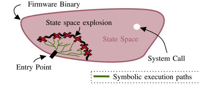
(a) Existing techniques start from the entry point, and fail before reaching the system call due to state space explosion.
